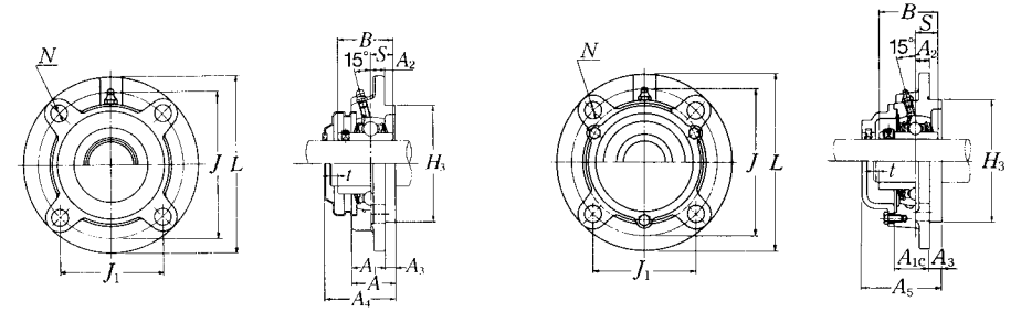
Pressed steel dust cover type Open end Z-UCFC...D1 Closed end ZM-UCFC...D1
