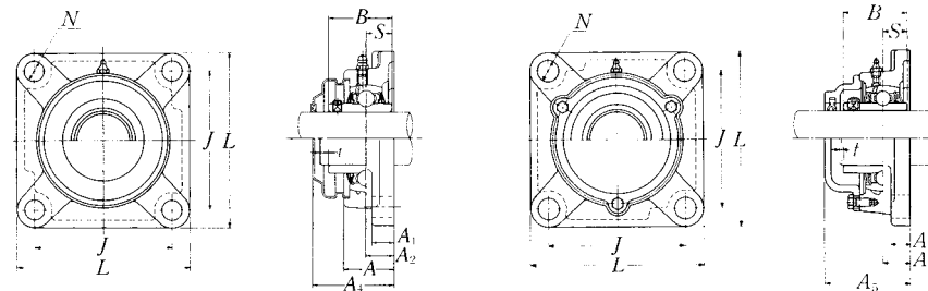
Pressed steel dust cover type Open end Z-UCF...D1 Closed end ZM-UCF...D1
