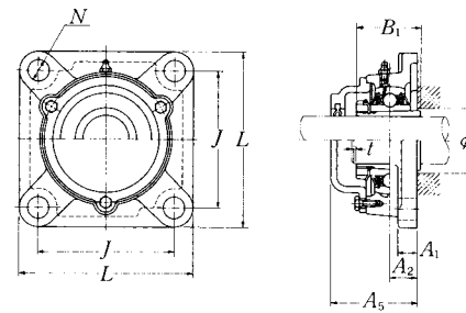
Cast dust cover type Open end C-UKF...D1 Closed end CM-UKF...D1
