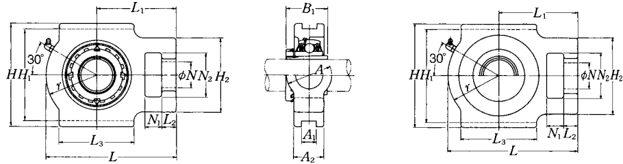
Pressed steel dust cover type Open end Z-UKT...D1 Closed end ZM-UKT...D1
