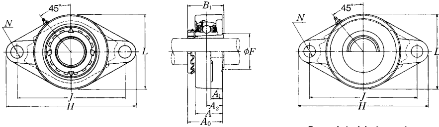
Pressed steel dust cover type Open end Z-UKFL...D1 Closed end ZM-UKFL...D1
