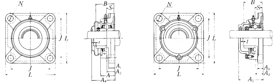
Pressed steel dust cover type Open end Z-UCF...D1 Closed end ZM-UCF...D1
