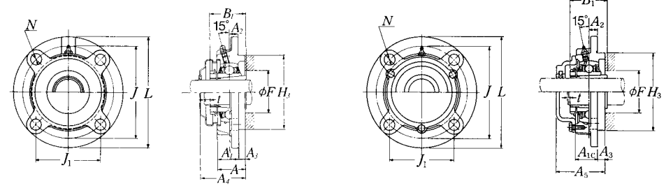
Pressed steel dust cover type Open end Z-UKFC...D1 Closed end ZM-UKFC...D1
