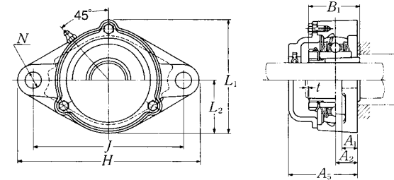
Cast dust cover type Open end C-UKFL...D1 Closed end CM-UKFL...D1
