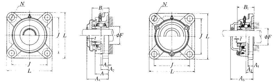
Pressed steel dust cover type Open end Z-UKF...D1 Closed end ZM-UKF...D1
