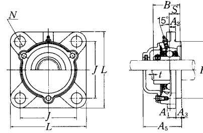
Cast dust cover type Open end C-UCFS...D1 Closed end CM-UCFS...D1
