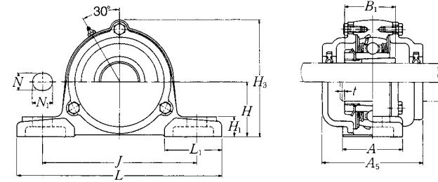
Cast dust cover type Open end C-UKP...D1 Closed end CM-UKP...D1
