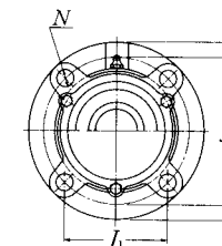
Cast dust cover type Open end C-UCFC...D1 Closed end CM-UCFC...D1
