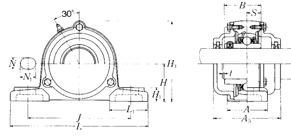
Cast dust cover type Open end C-UCP...D1 Closed end CM-UCP...D1
