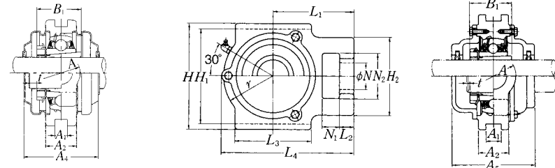
Cast dust cover type Open end C-UKT...D1 Closed end CM-UKT...D1
