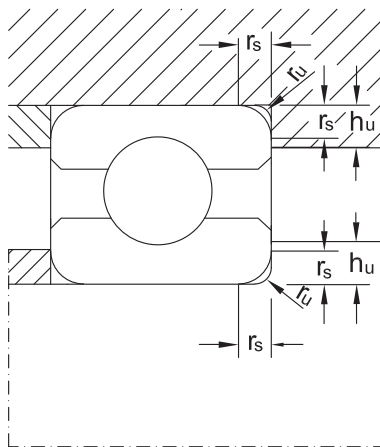
Abutment dimensions
