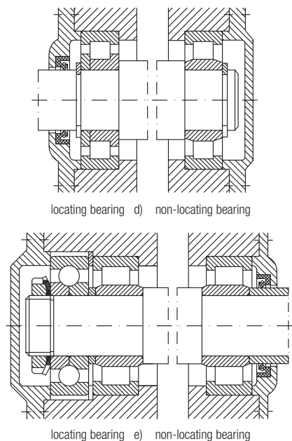
locating bearing e) non-locating bearing
