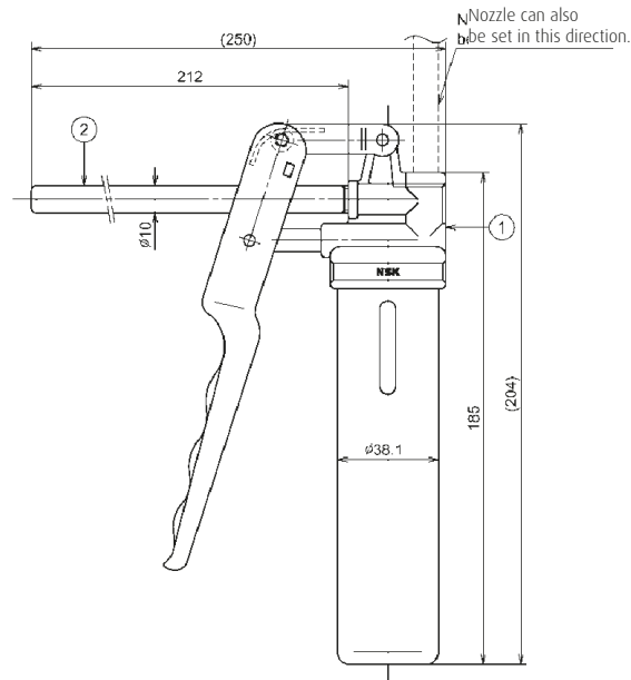
Fig I.7 NSK Hand Grease Pump with NSK straight nozzle
