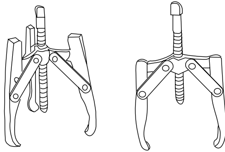
Bearing Pullers
